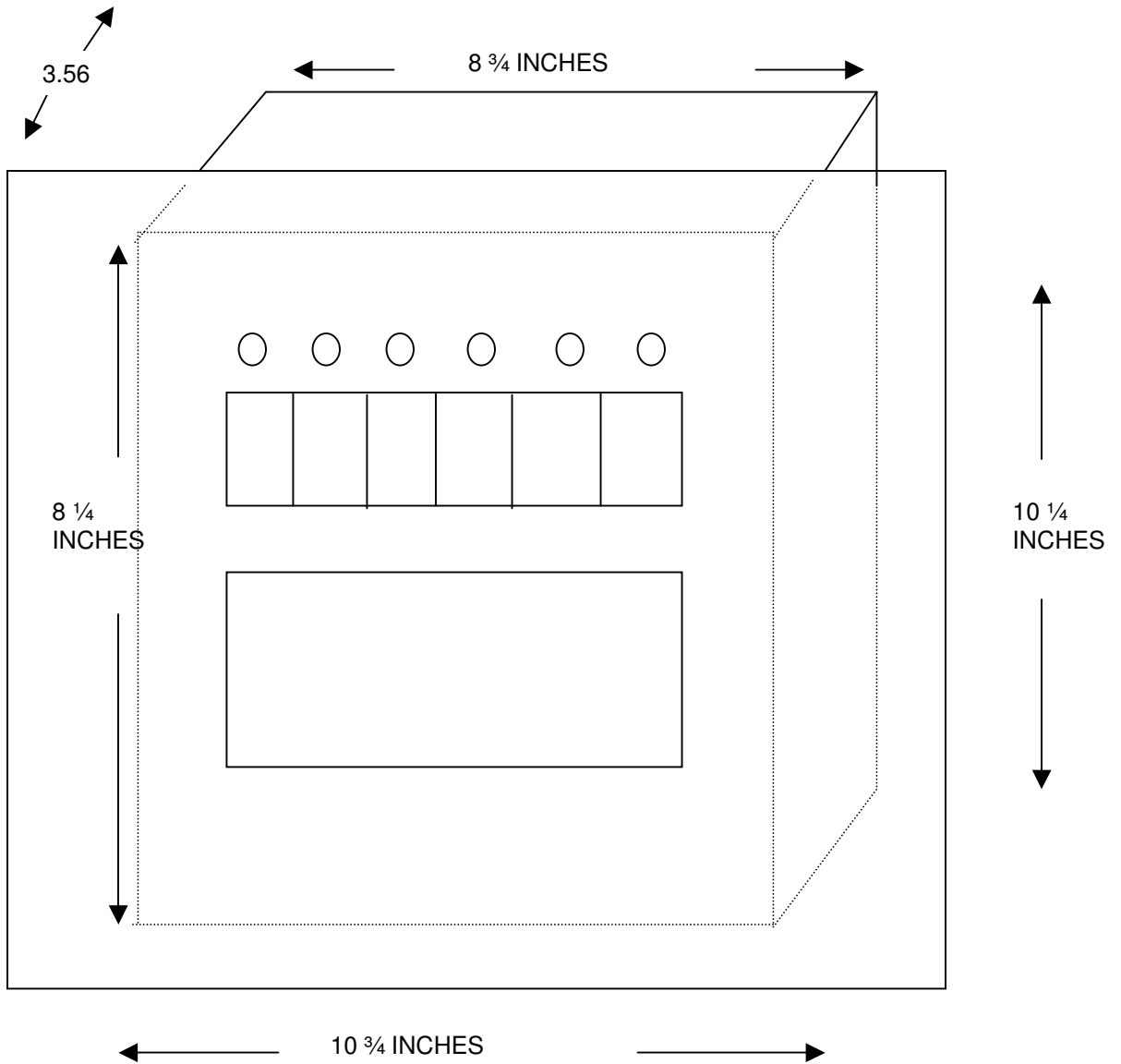
IDS 440 PANEL MOUNT DIMENSIONS
